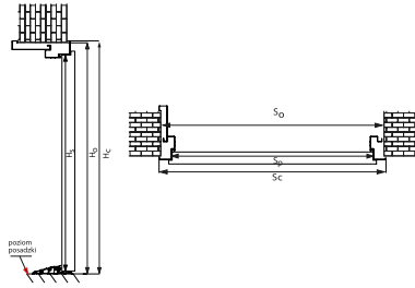
How to take the dimensions of IRON doors with corner frame
