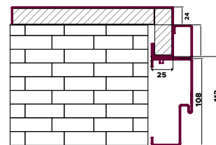
PORTAL WITH IRON ADJUSTABLE FRAME
