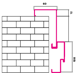
Architrave with the IRON internal door frame
