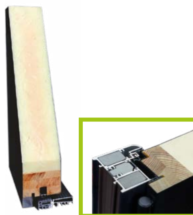
WMPTPL TERMO PRESTIGE LUX
